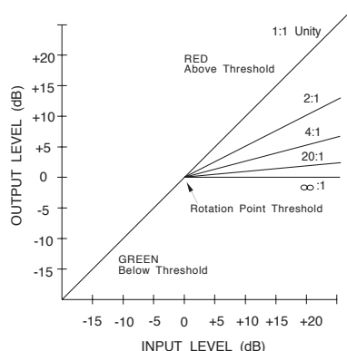
Figure 1 : Mode de compression Hard Knee
