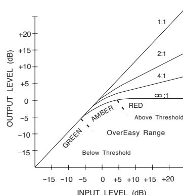
Figure 2 : Mode de compression OverEasy
